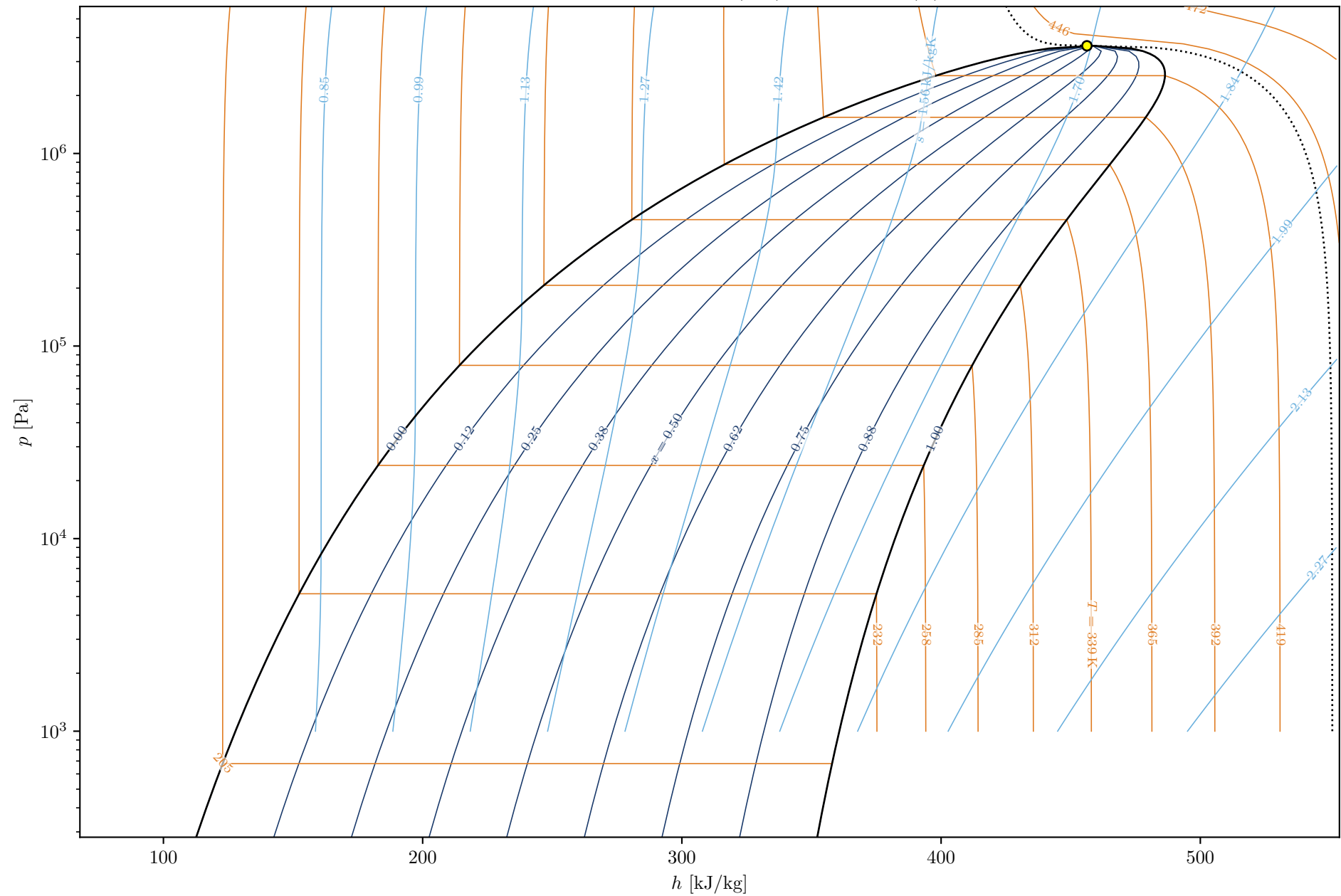
Thermodynamic Diagram (PH) — R1233zd(E)
